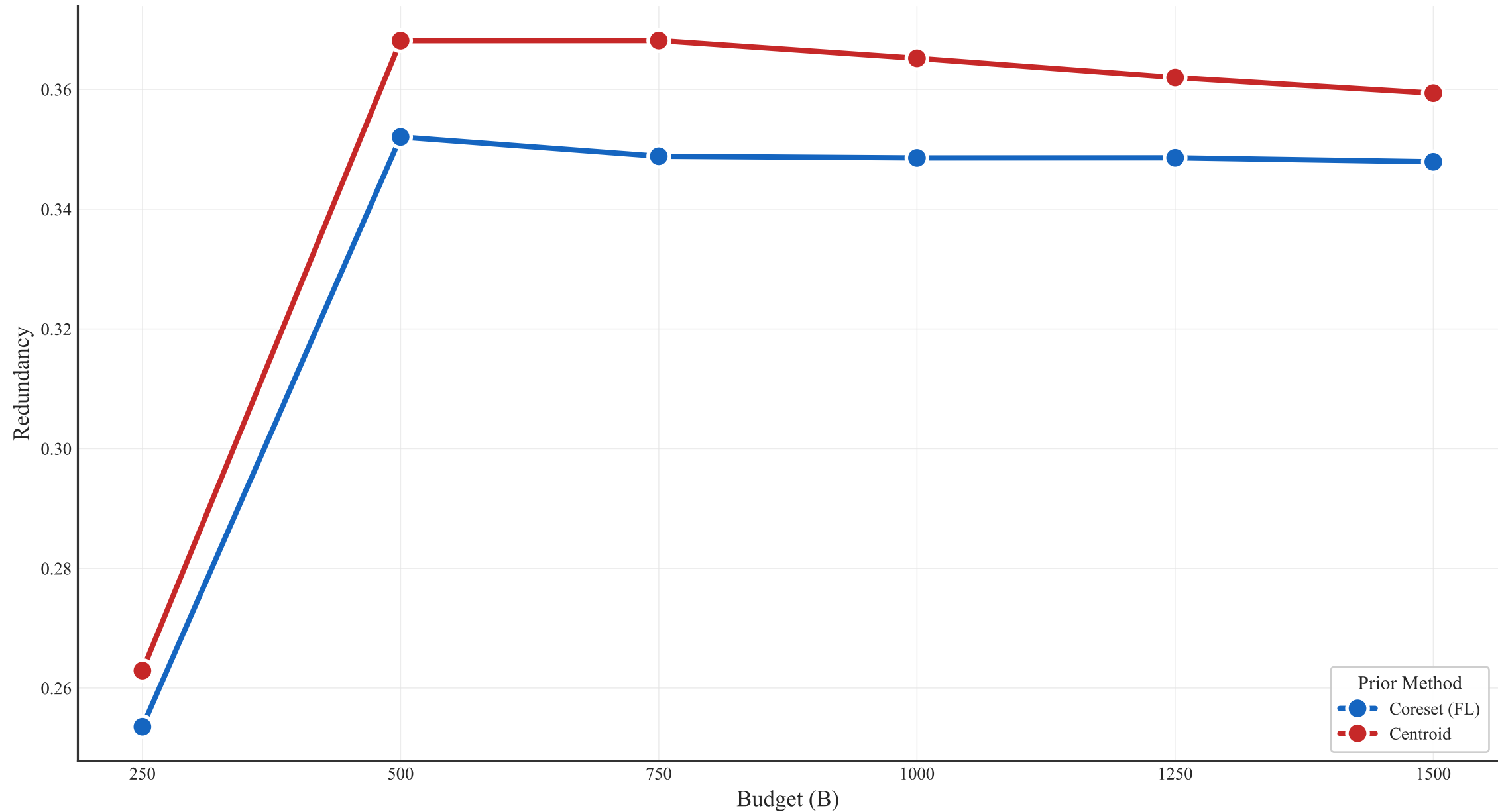
Centroid vs Coreset: Redundancy
