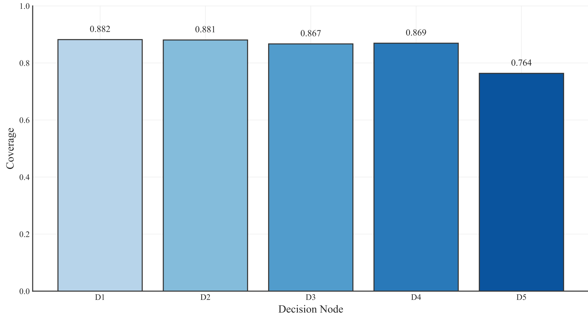
BGE-M3: Decision Coverage Breakdown (B=1000, Coreset (FL), prior/fl/cost_norm)
