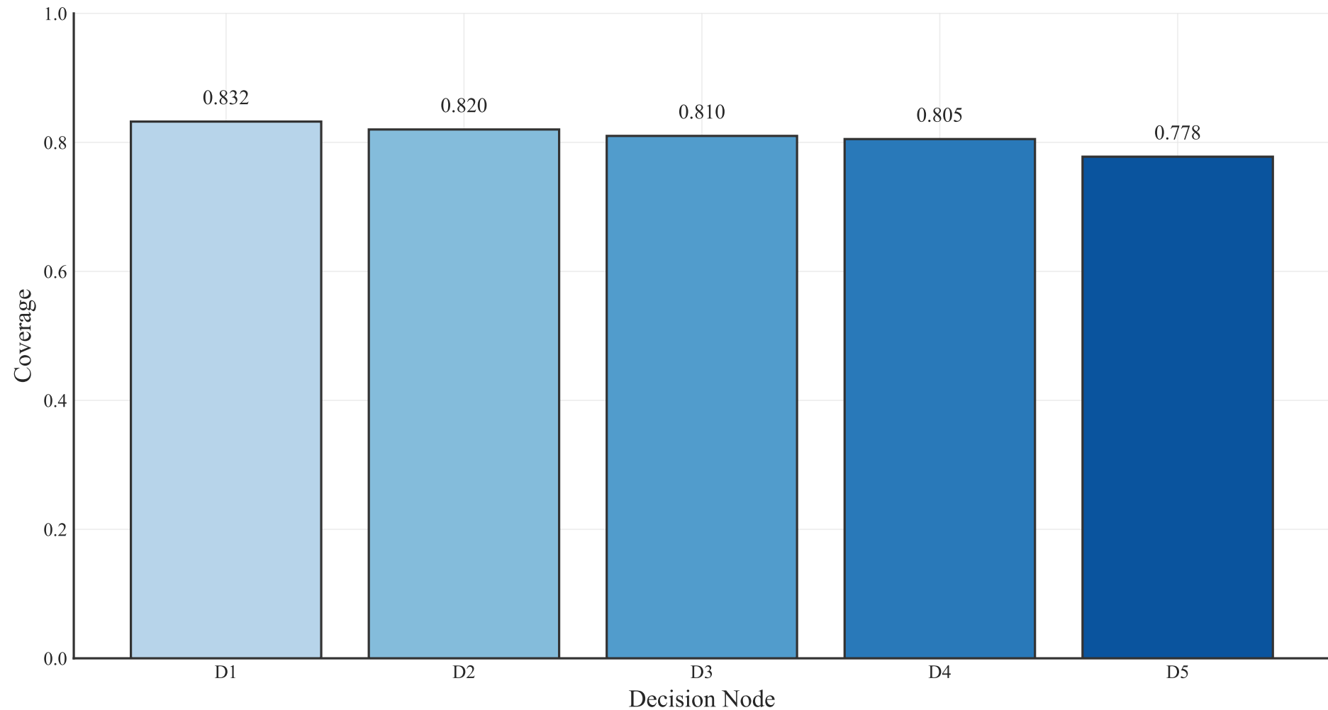
Gemma-300M: Decision Coverage Breakdown (B=1000, Coreset (FL), prior/fl/cost_norm)
