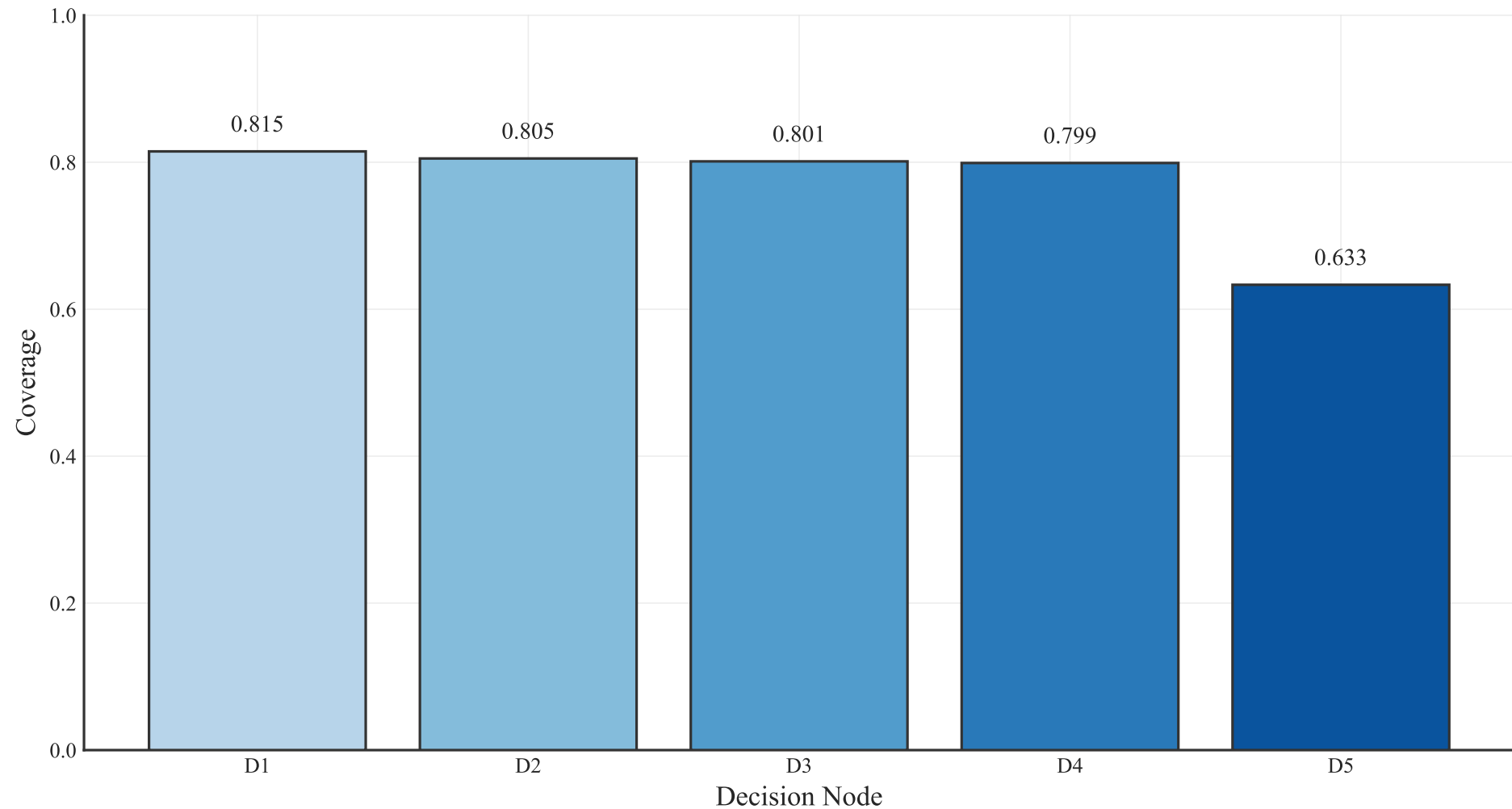
MPNet: Decision Coverage Breakdown (B=1000, Coreset (FL), prior/fl/cost_norm)
