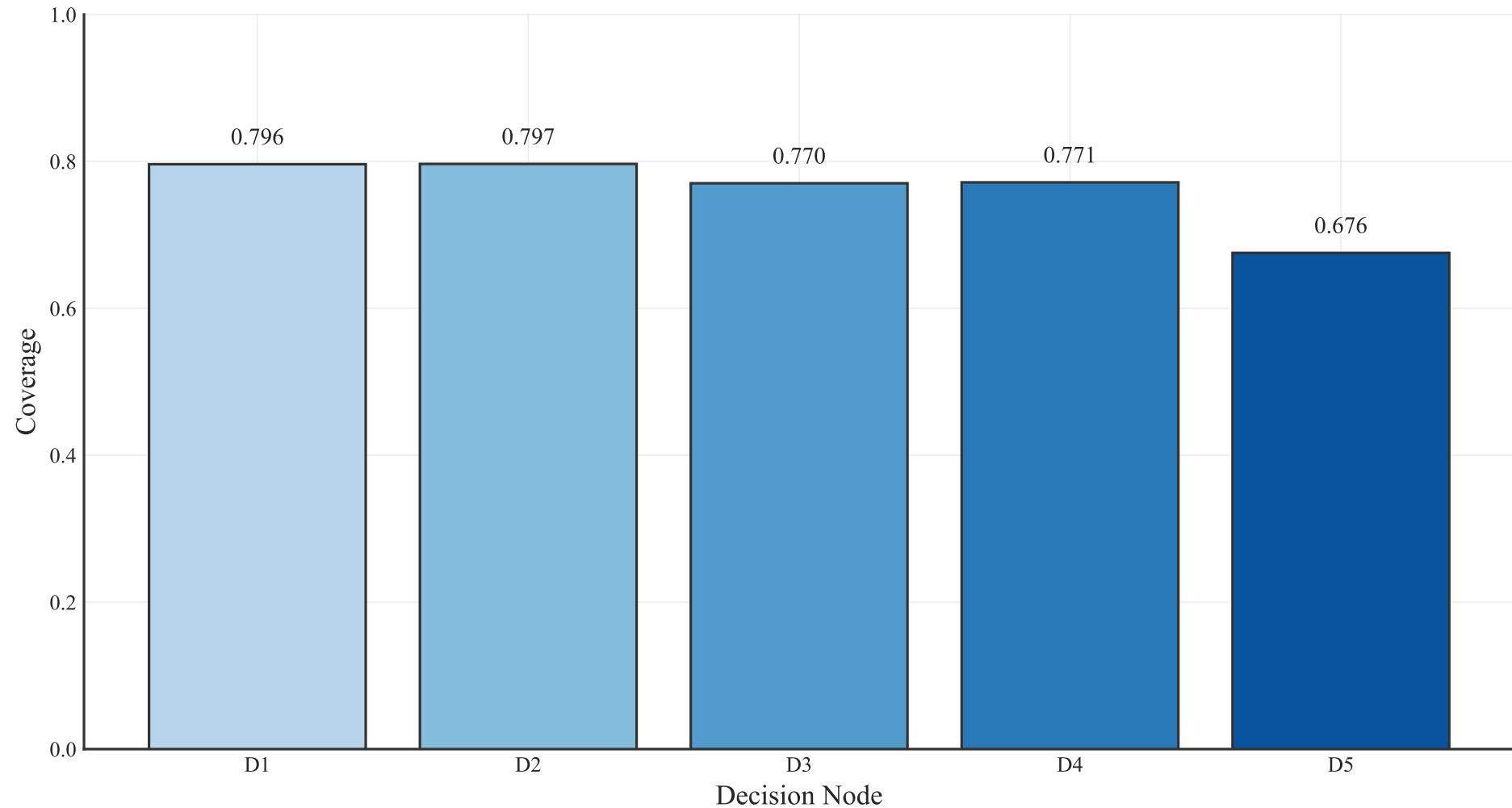
MiniLM-L6: Decision Coverage Breakdown (B=1000, Coreset (FL), prior/fl/cost_norm)
