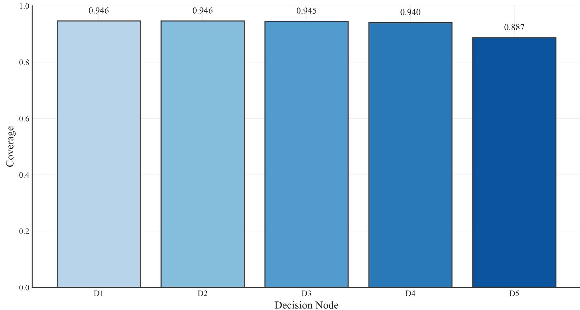
Qwen-0.6B: Decision Coverage Breakdown (B=1000, Coreset (FL), prior/fl/cost_norm)
