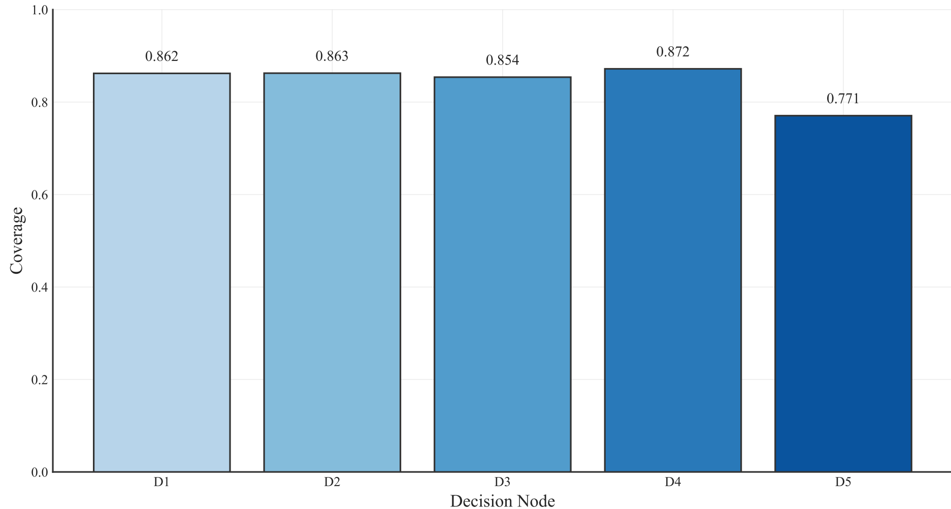
Stella-1.5B: Decision Coverage Breakdown (B=1000, Coreset (FL), prior/fl/cost_norm)
