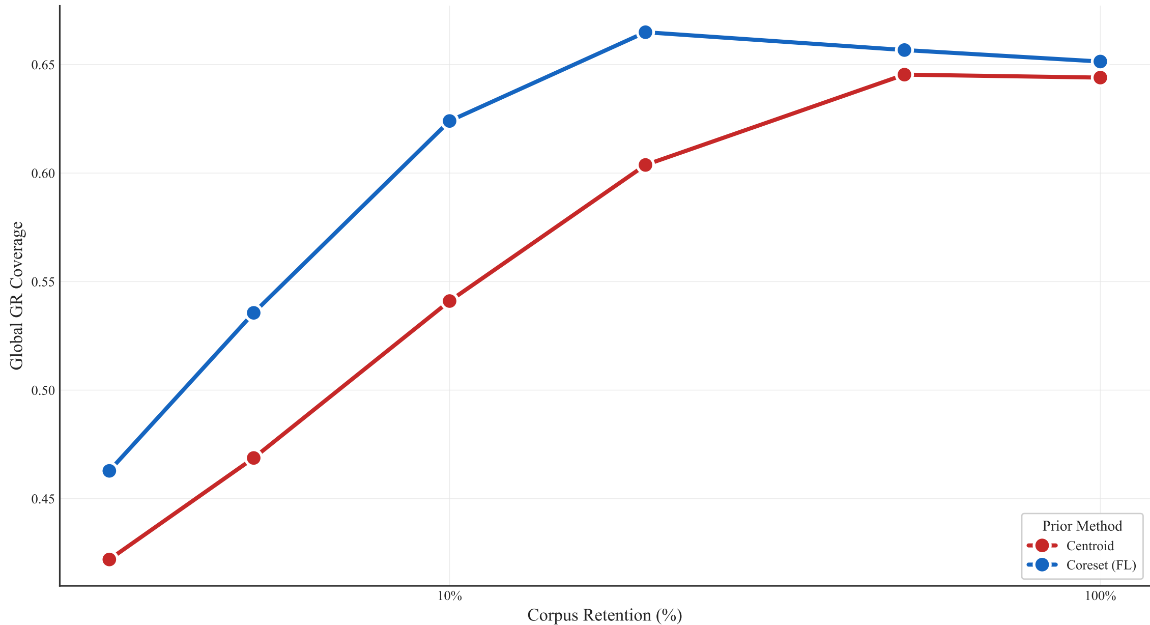
Filtering: Centroid vs Coreset — Global GR Coverage
