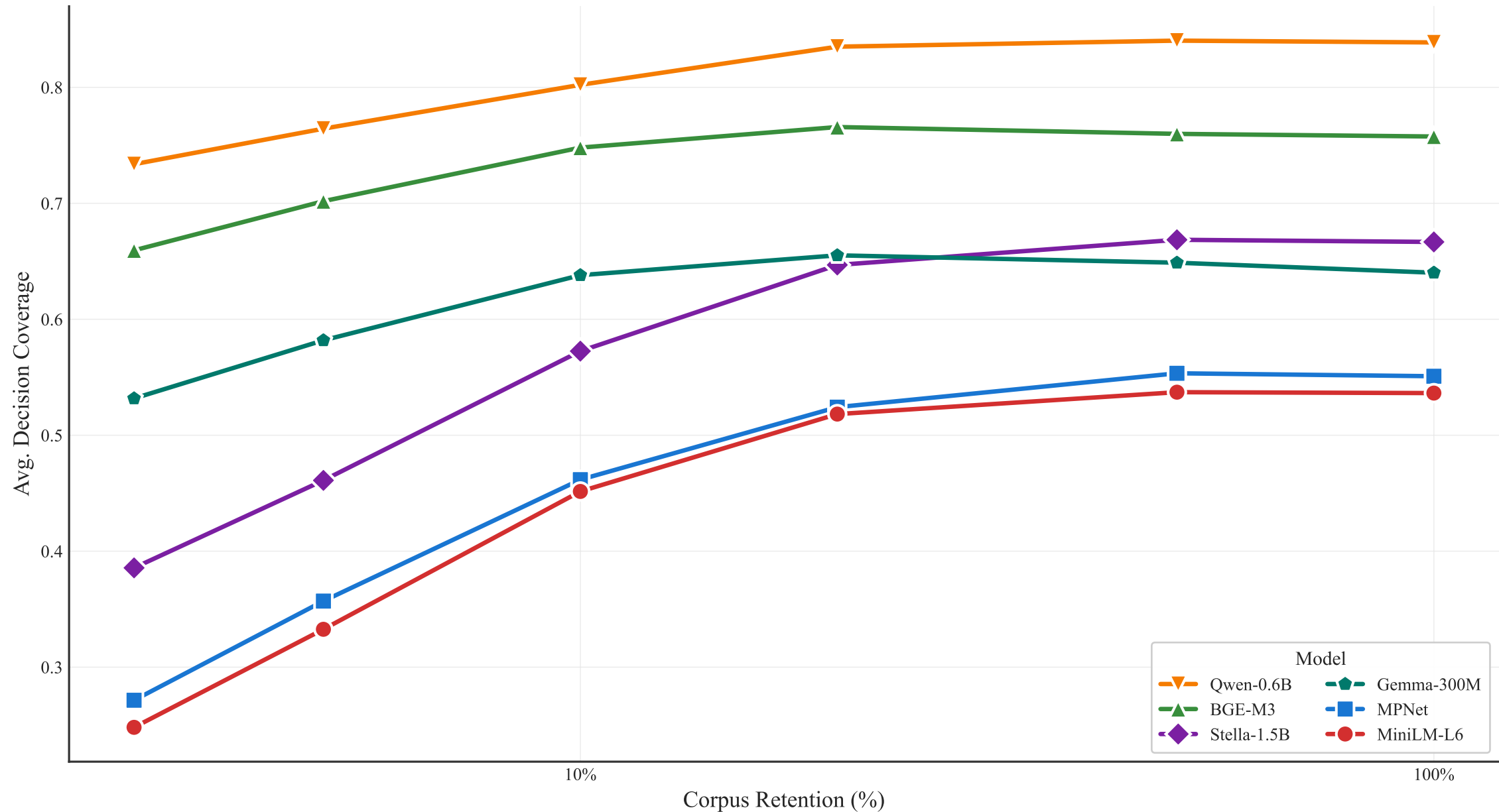
Corpus Filtering: Avg. Decision Coverage vs Retention
