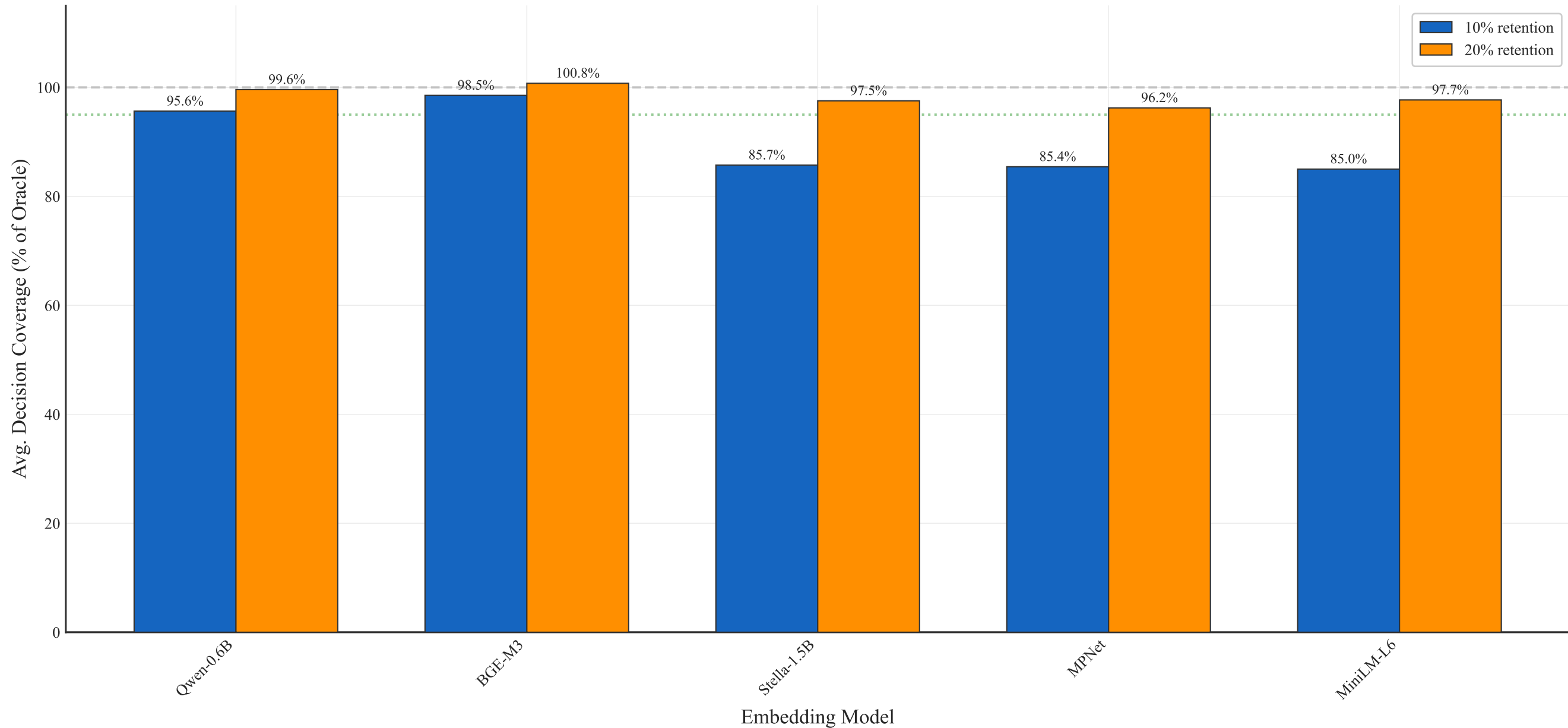
Filtering Efficiency: Avg. Decision Coverage Retained at 10% and 20% Corpus
