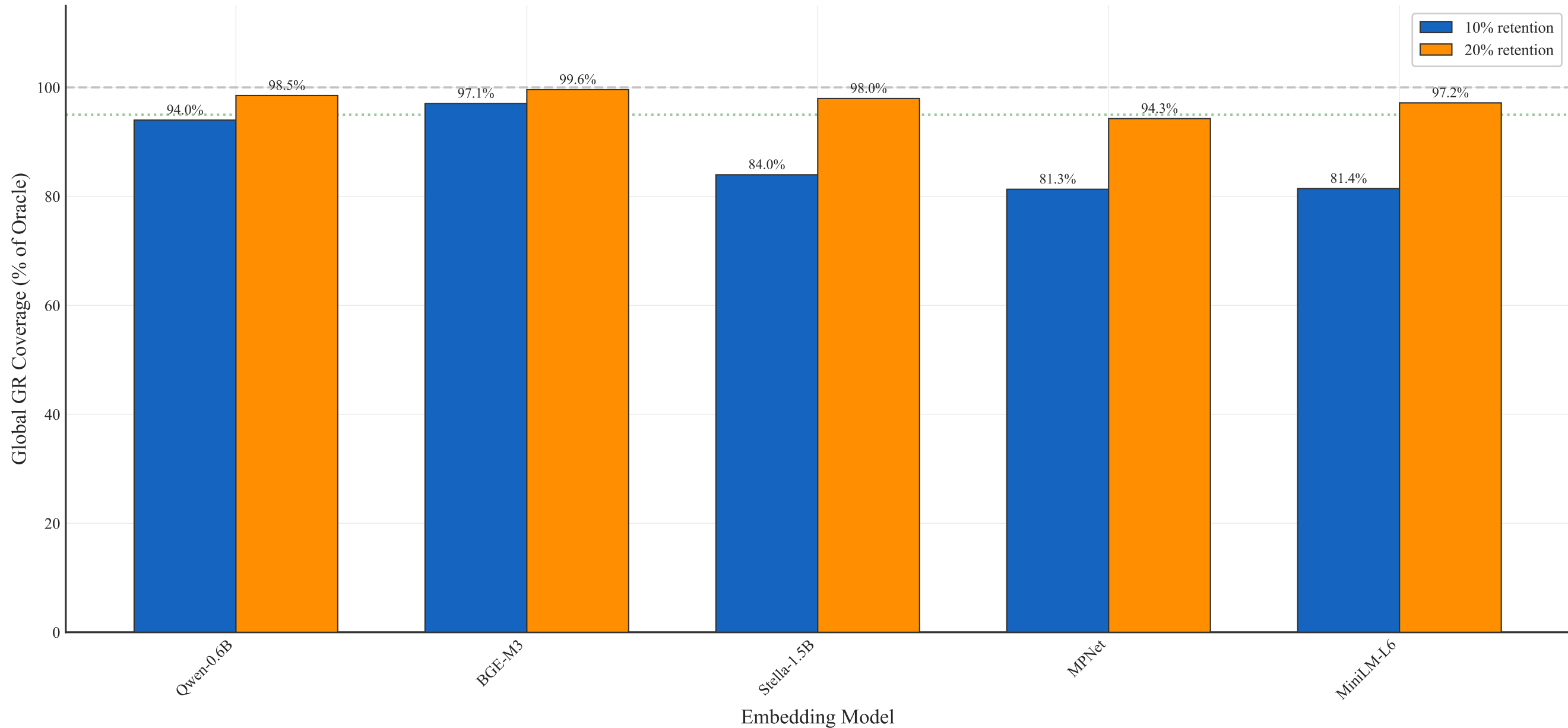
Filtering Efficiency: Global GR Coverage Retained at 10% and 20% Corpus
