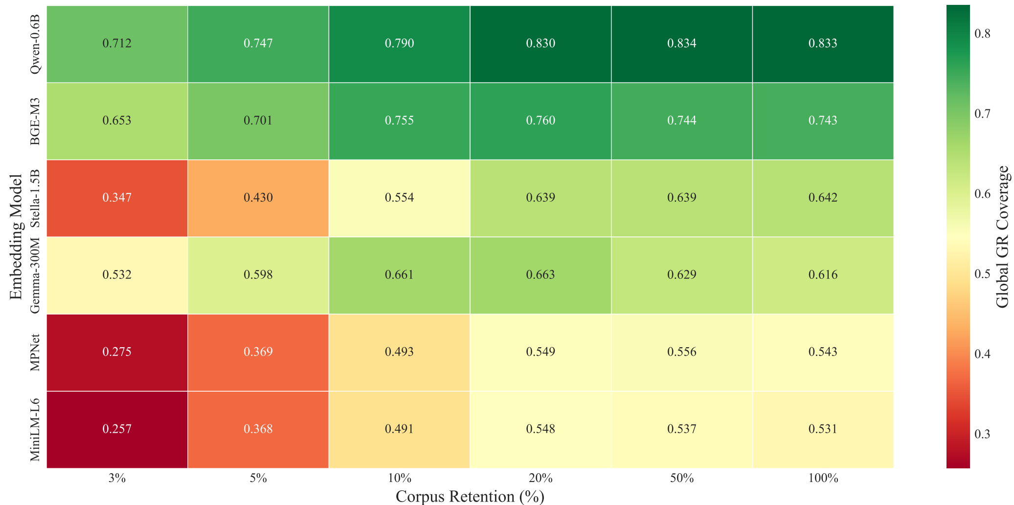
Global GR Coverage by Model &amp; Retention % — Coreset (FL)
