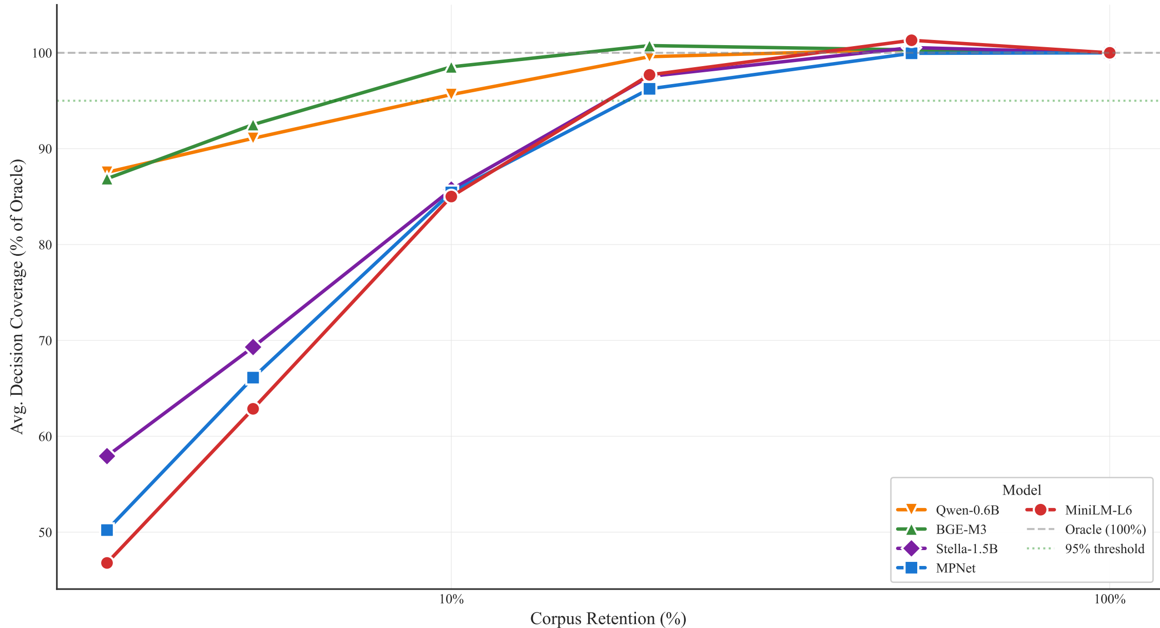
Normalized Avg. Decision Coverage: Degradation from Filtering
