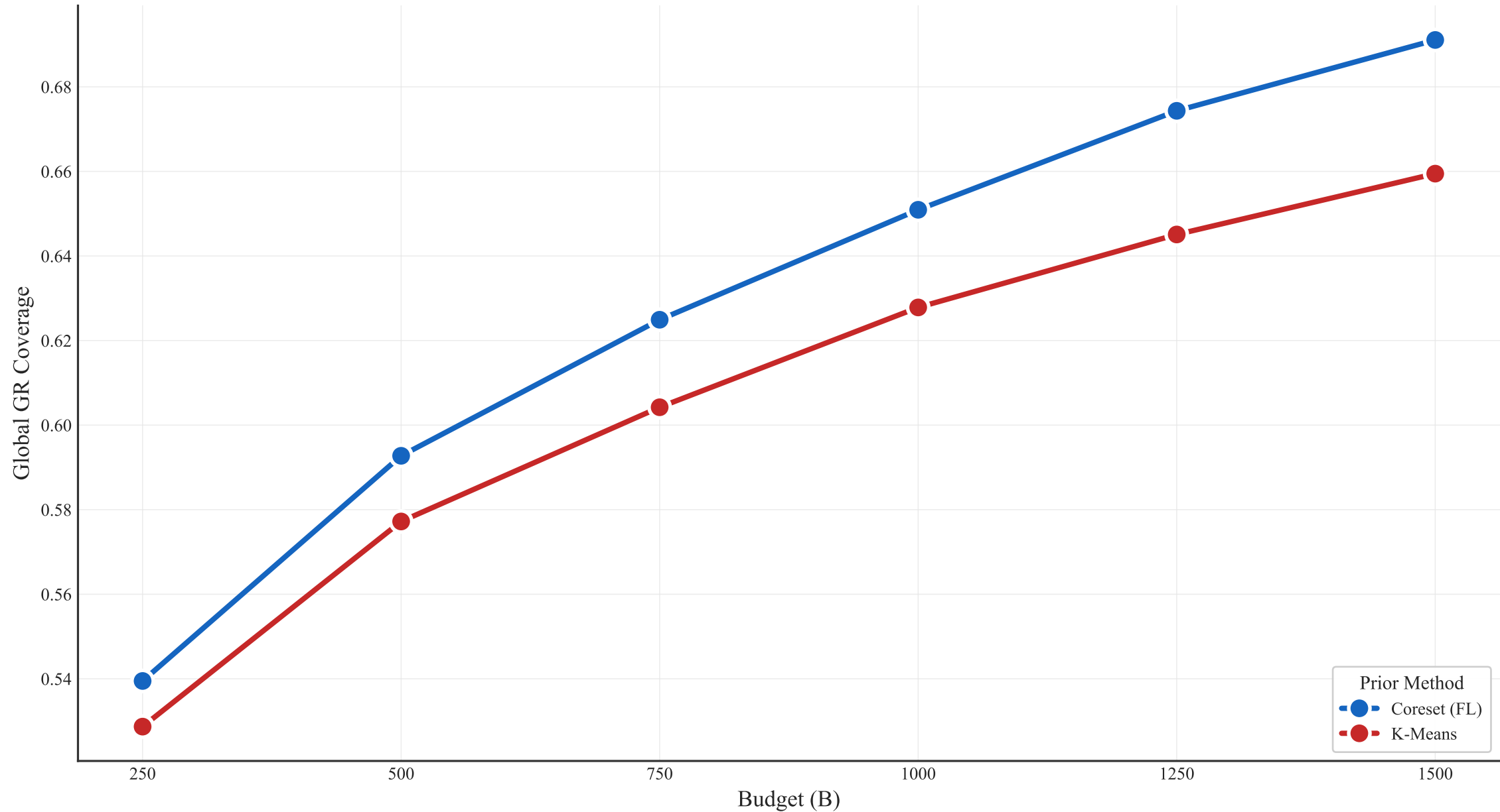
K-Means vs Coreset: Global GR Coverage
