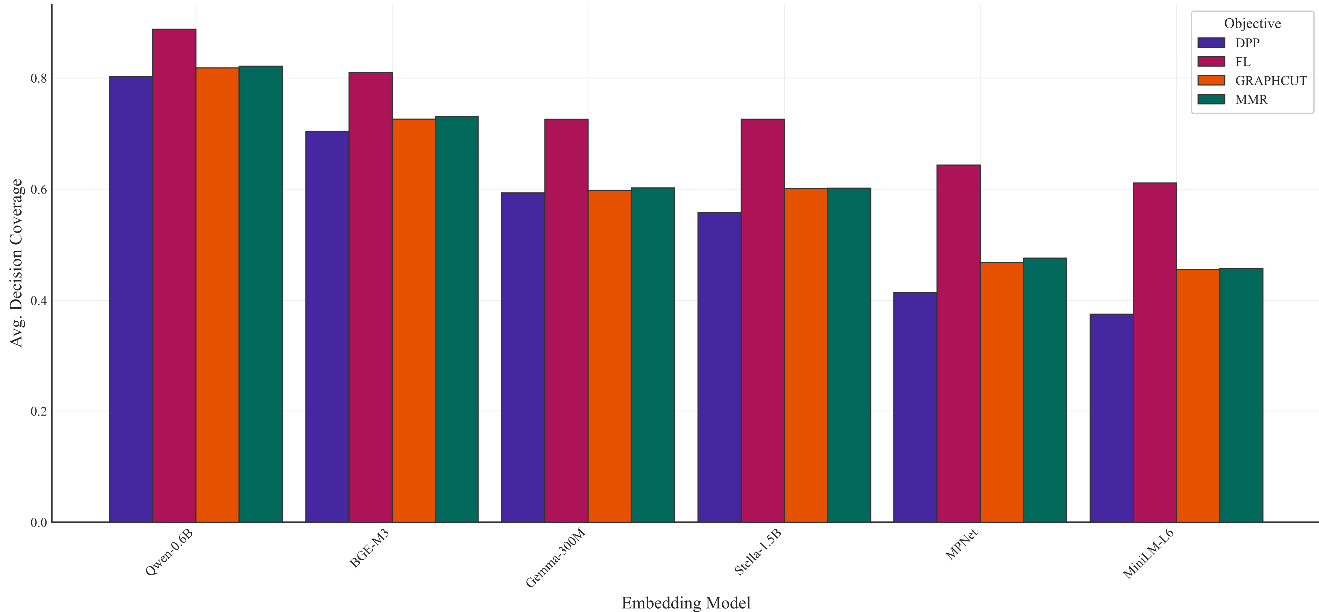
Model Performance by Objective (B=1000) — Centroid
