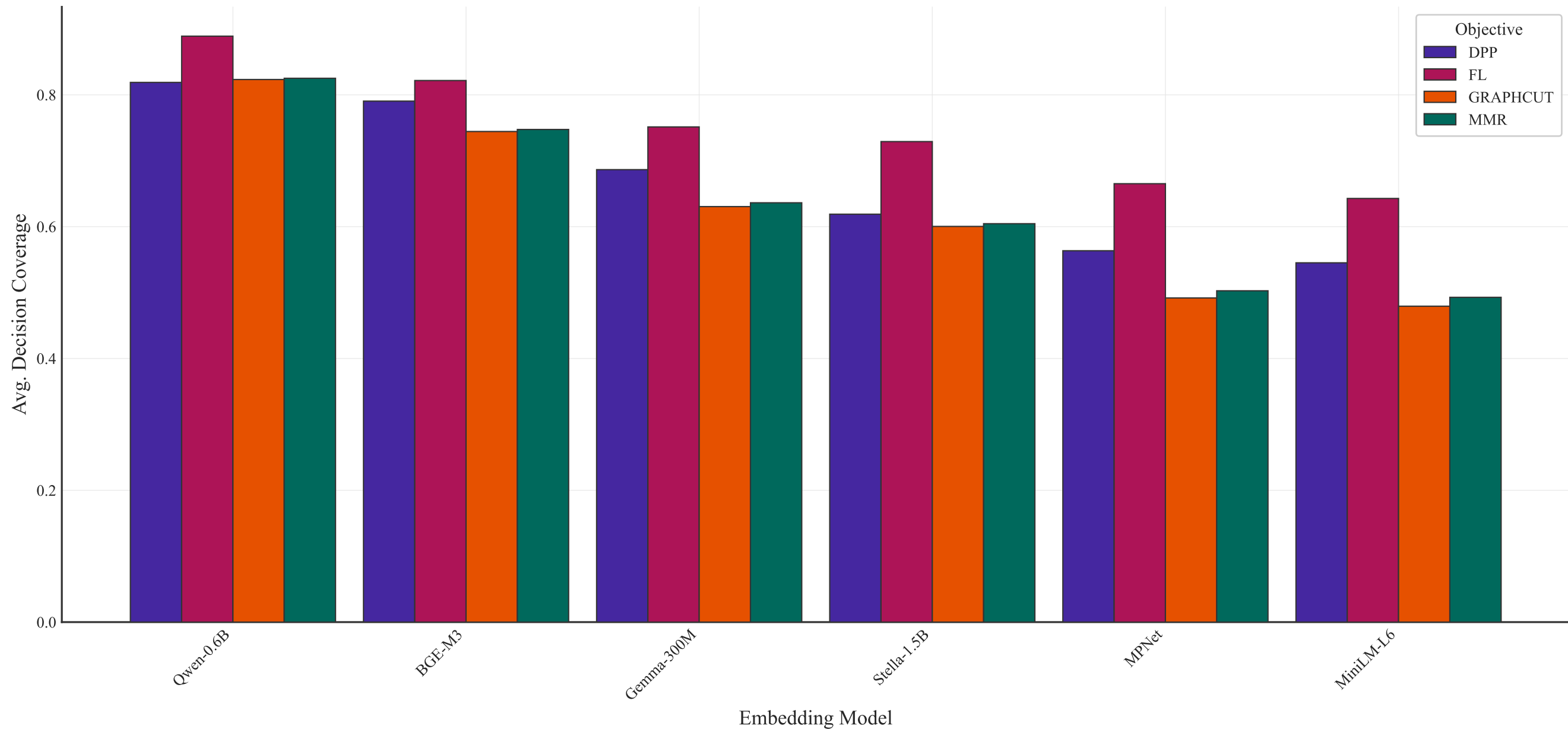
Model Performance by Objective (B=1000) — Coreset (FL)
