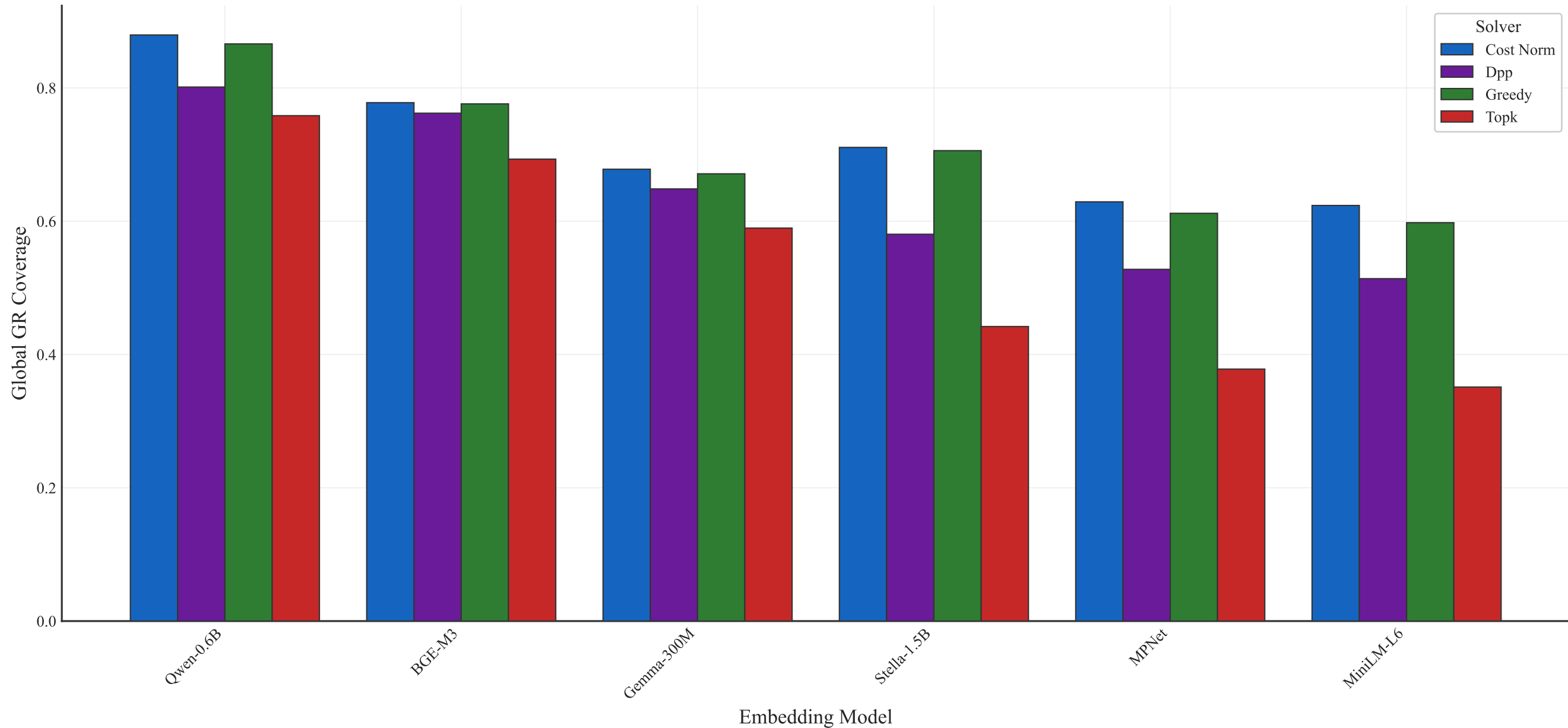
Model Performance by Solver (B=1000) — Coreset (FL)
