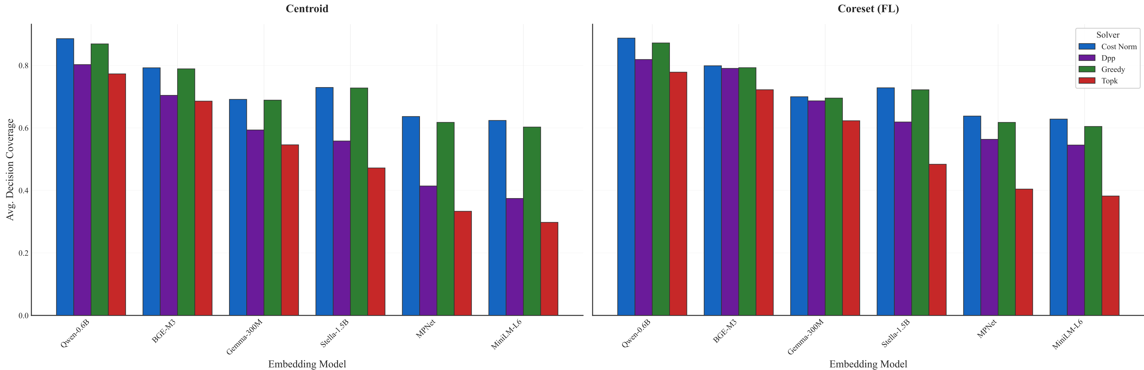
Avg. Decision Coverage by Solver (B=1000)
