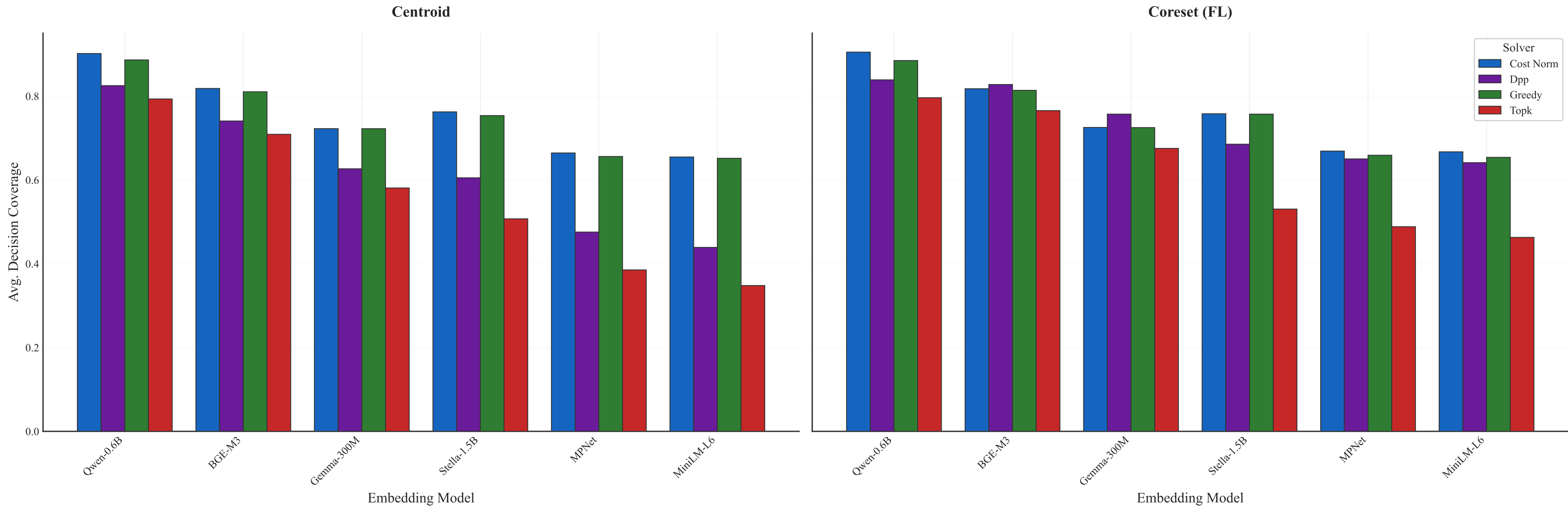
Avg. Decision Coverage by Solver (B=1500)
