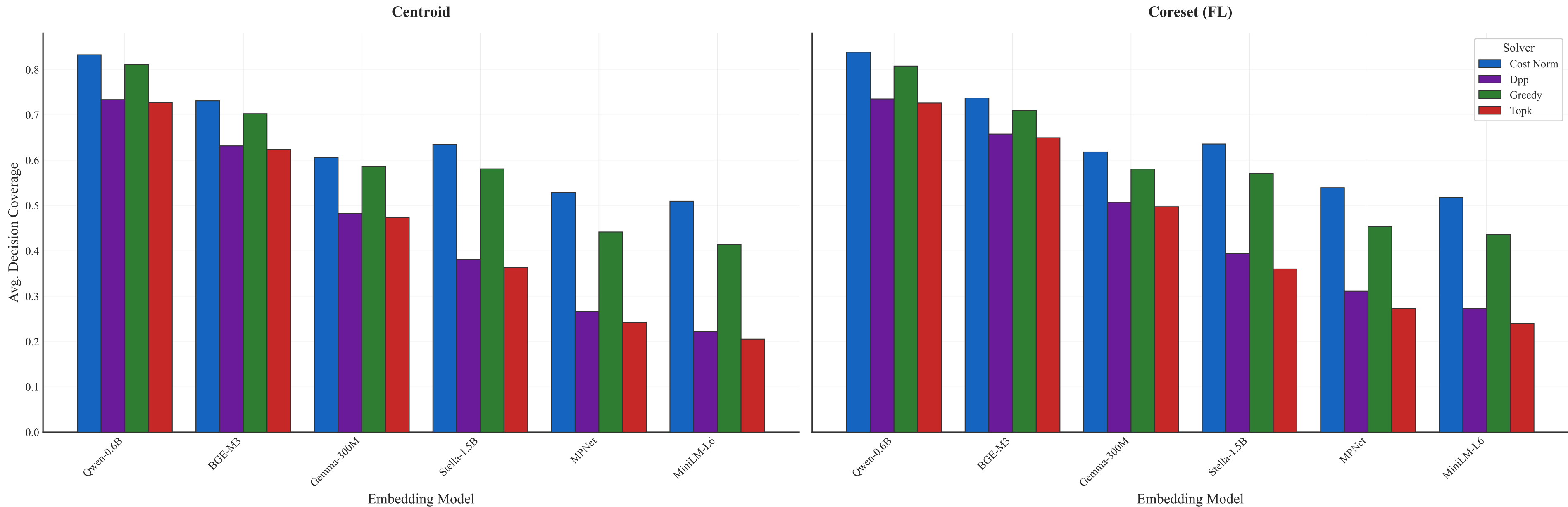
Avg. Decision Coverage by Solver (B=250)
