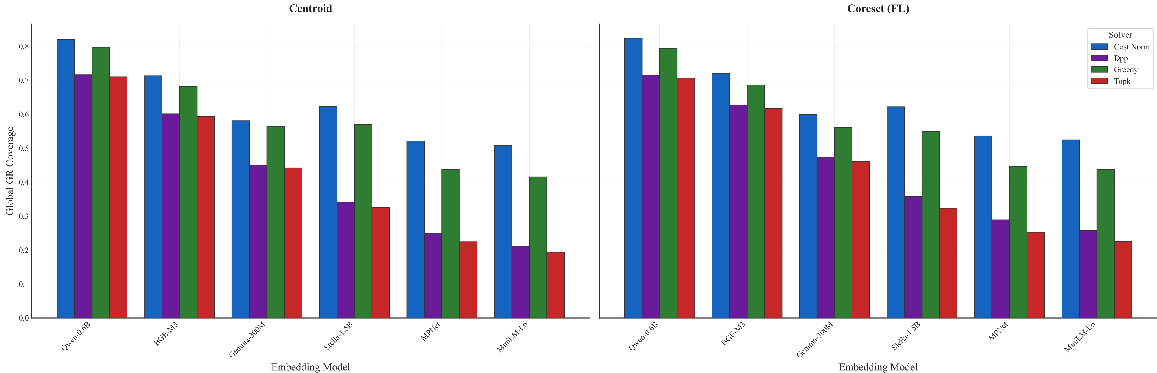
Global GR Coverage by Solver (B=250)
