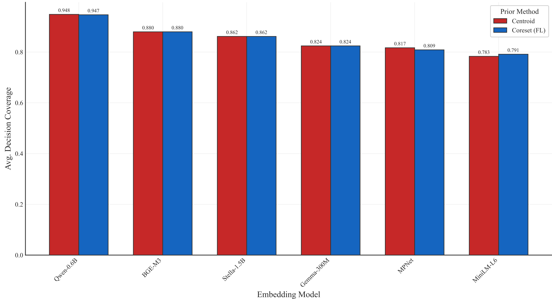
Centroid vs Coreset by Model (B=1000)
