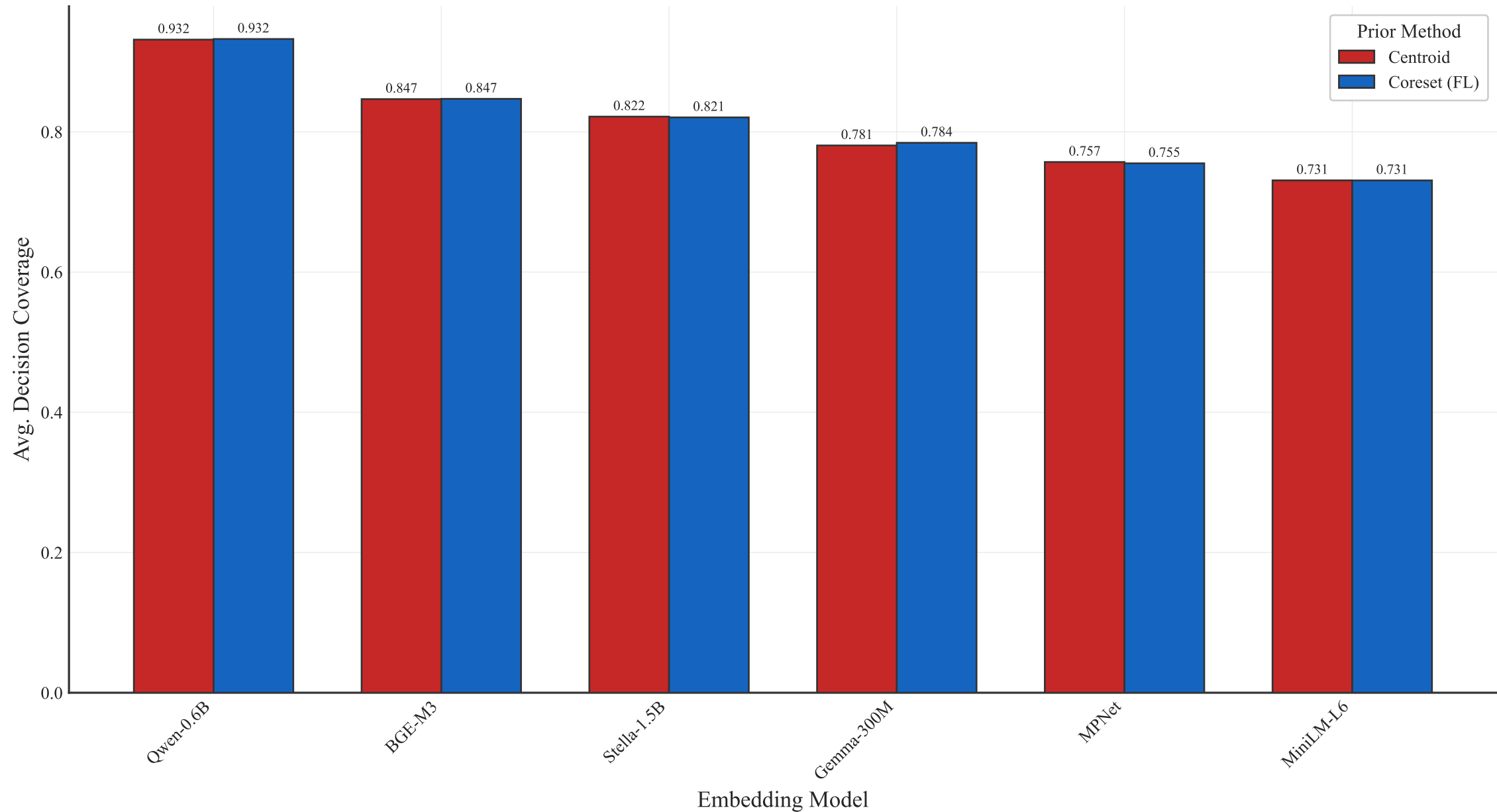
Centroid vs Coreset by Model (B=500)
