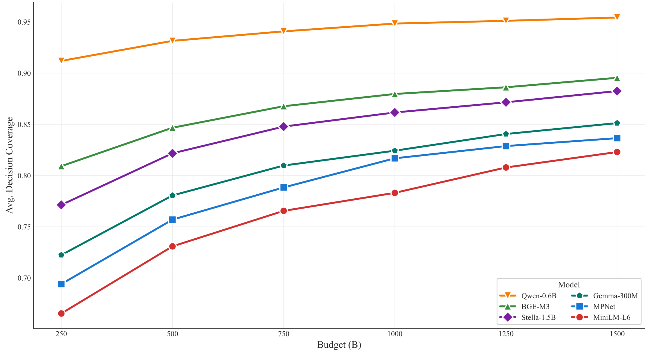
Model Comparison: Avg. Decision Coverage (Centroid)
