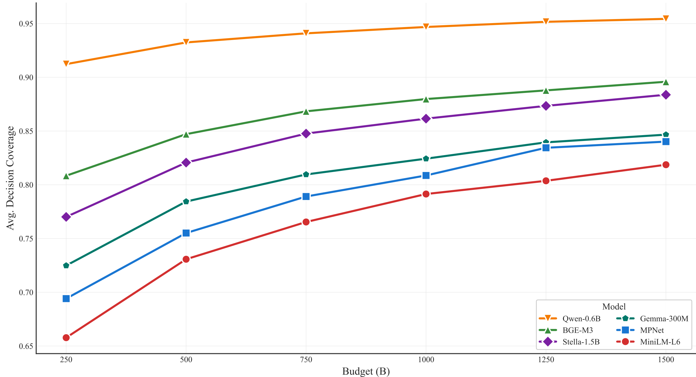
Model Comparison: Avg. Decision Coverage (Coreset (FL))
