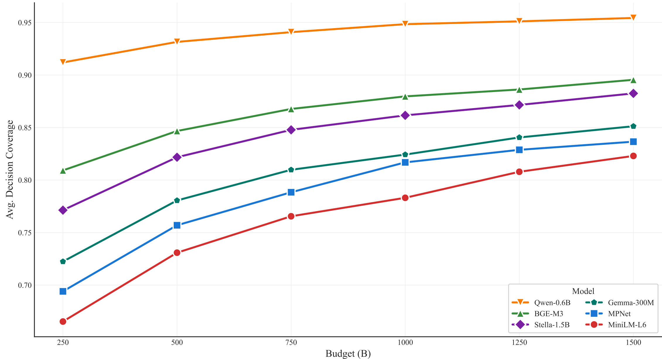
Model Comparison: Avg. Decision Coverage (K-Means)
