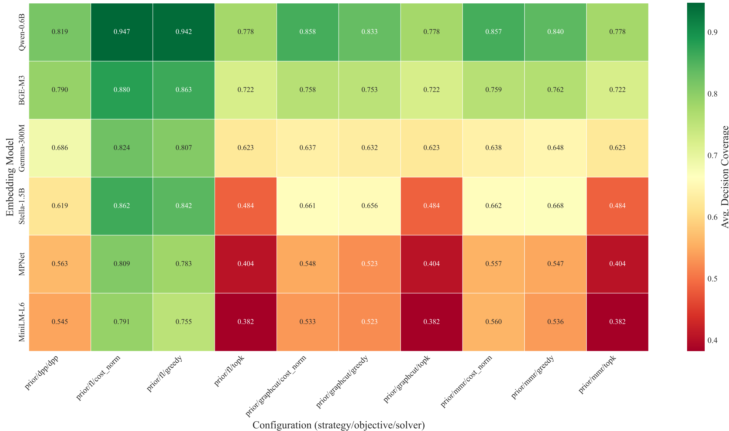
Avg. Decision Coverage by Model & Config (B=1000) — Coreset (FL)
