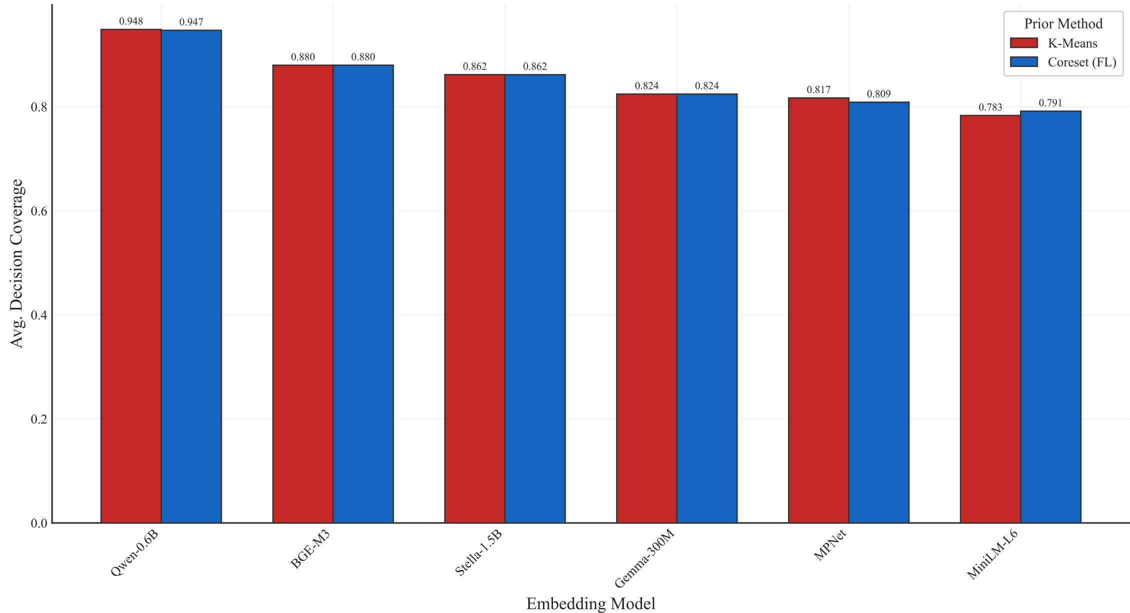
K-Means vs Coreset by Model (B=1000)
