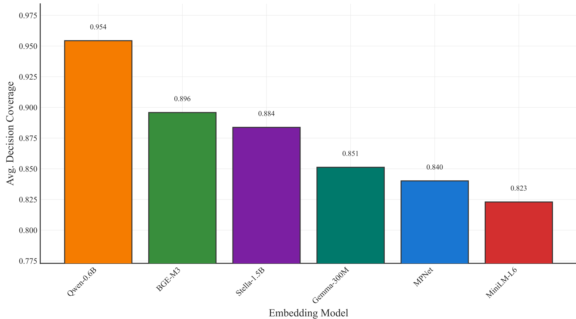
Model Ranking: Avg. Decision Coverage (B=1500)
