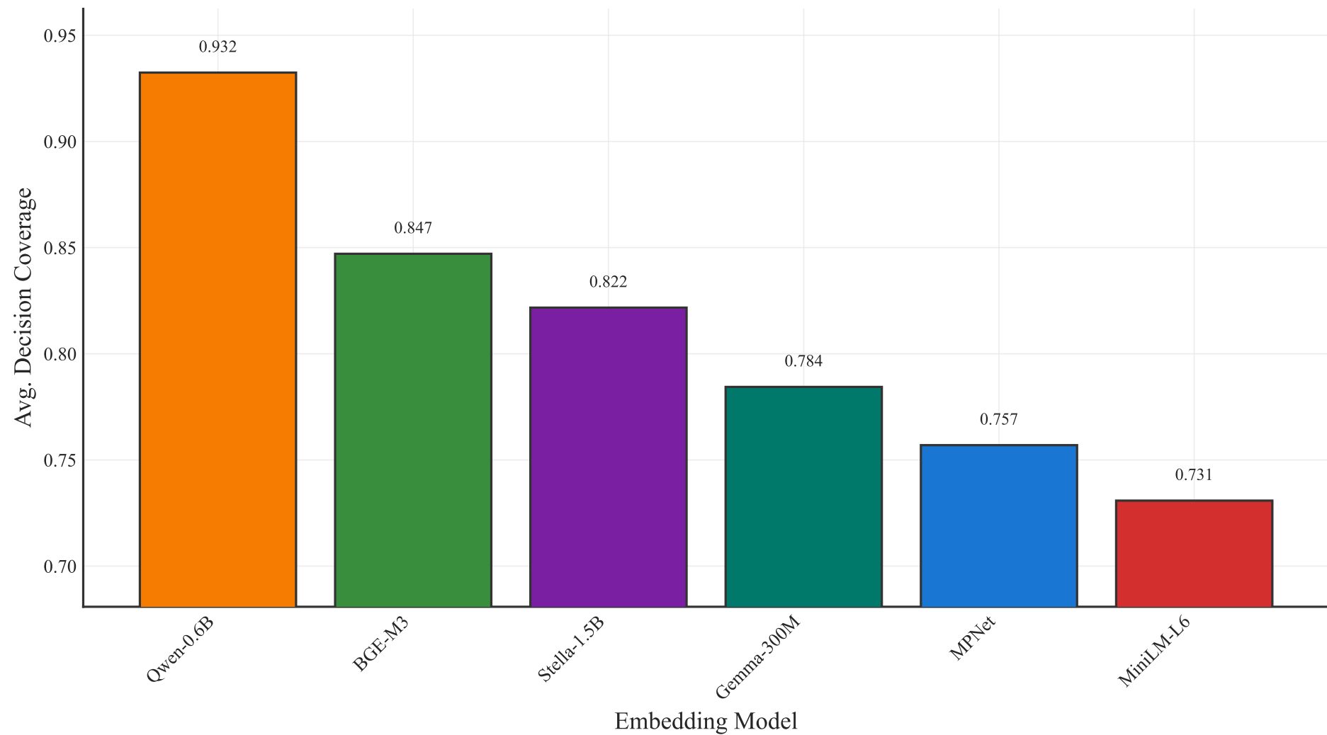
Model Ranking: Avg. Decision Coverage (B=500)
