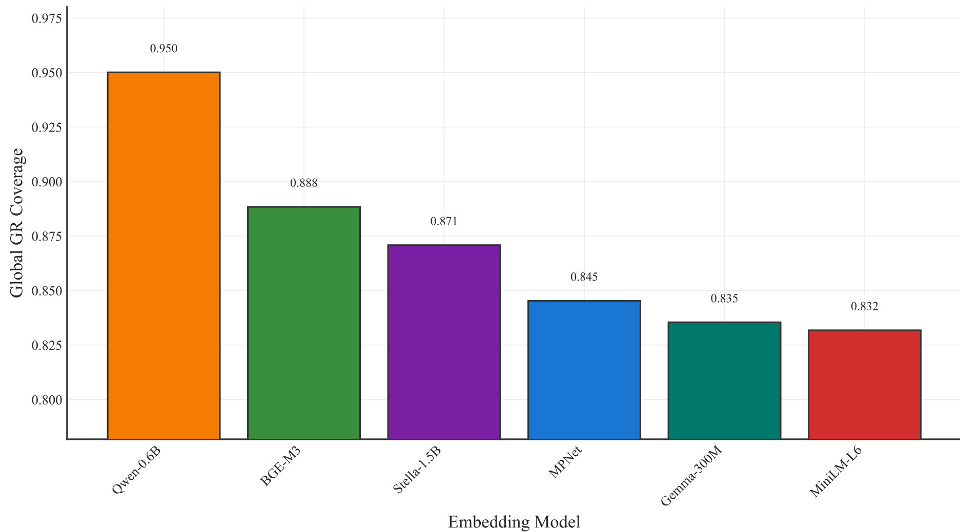
Model Ranking: Global GR Coverage (B=1500)
