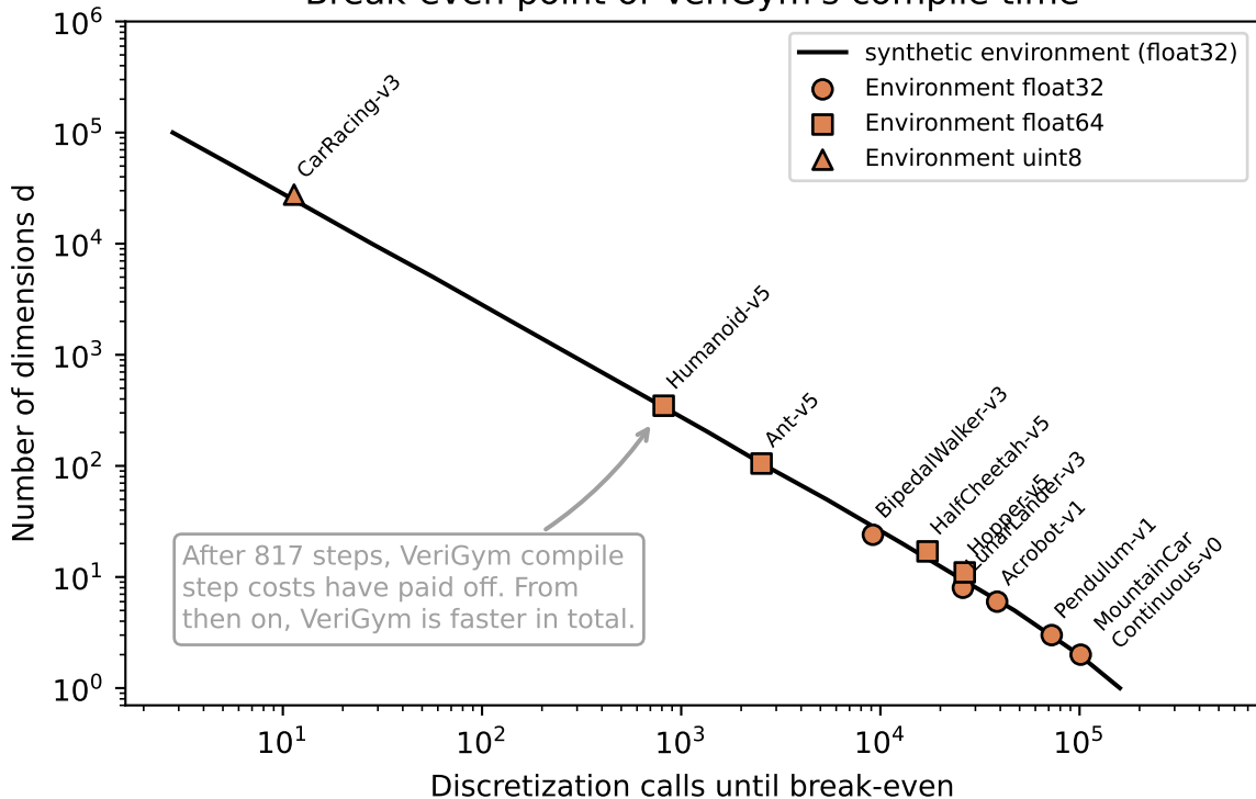
Break-even point of VeriGym's compile time
