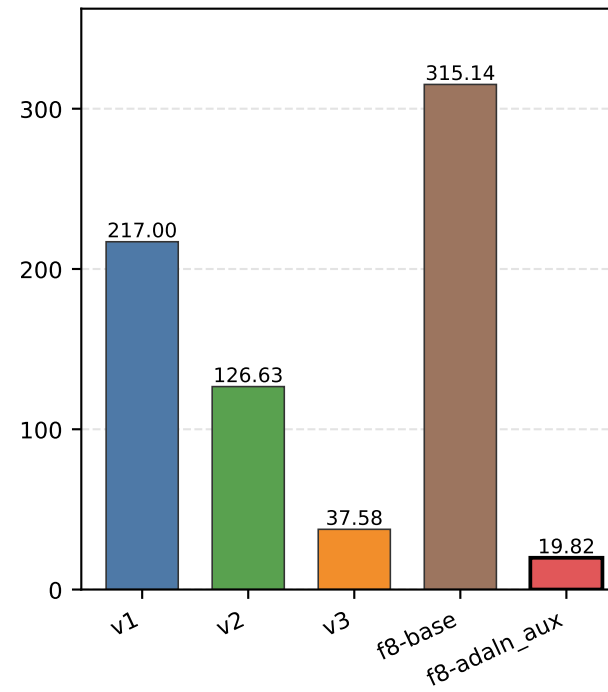
FID \downarrow
