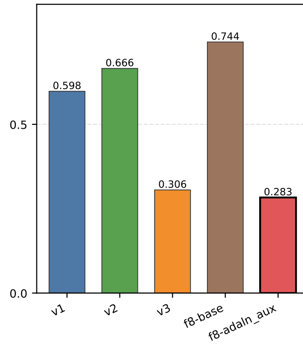
LPIPS \downarrow
