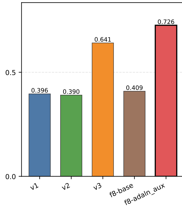
SSIM \uparrow
