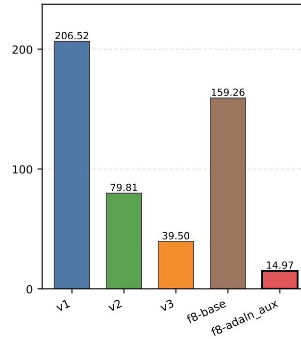
FVD \downarrow
