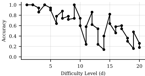
(b) Accuracy Curve
