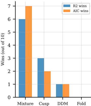
(a) Model Selection Wins
