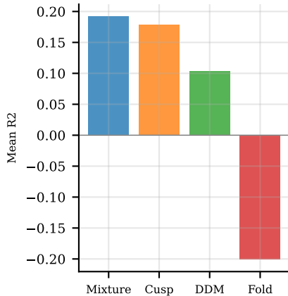
(b) Mean R2 Across Series
