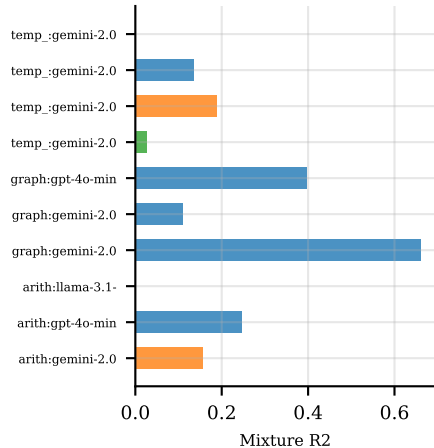
(c) Per-Series Mixture R2
