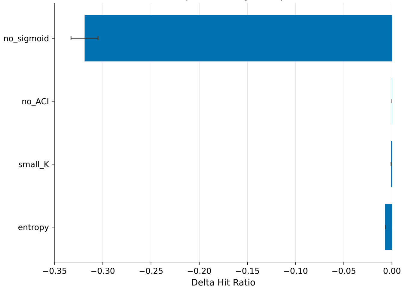
Ablation: Impact of Design Components
