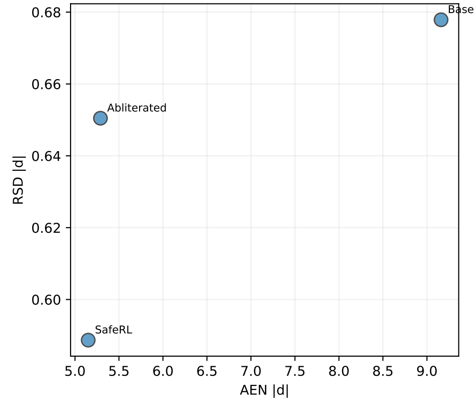
Activation Entropy (AEN) vs Residual Standard Deviation (RSD) r=0.757 , p=0.453
