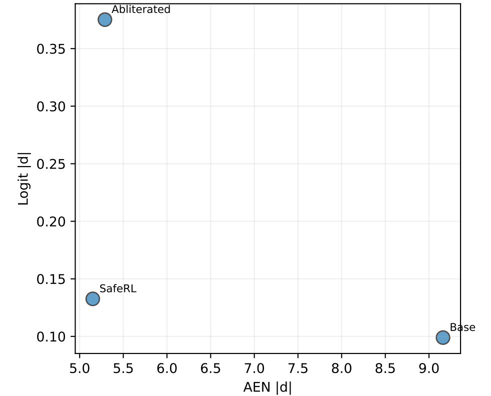
Activation Entropy (AEN) vs Logit-Gap Baseline r=-0.569 , p=0.615
