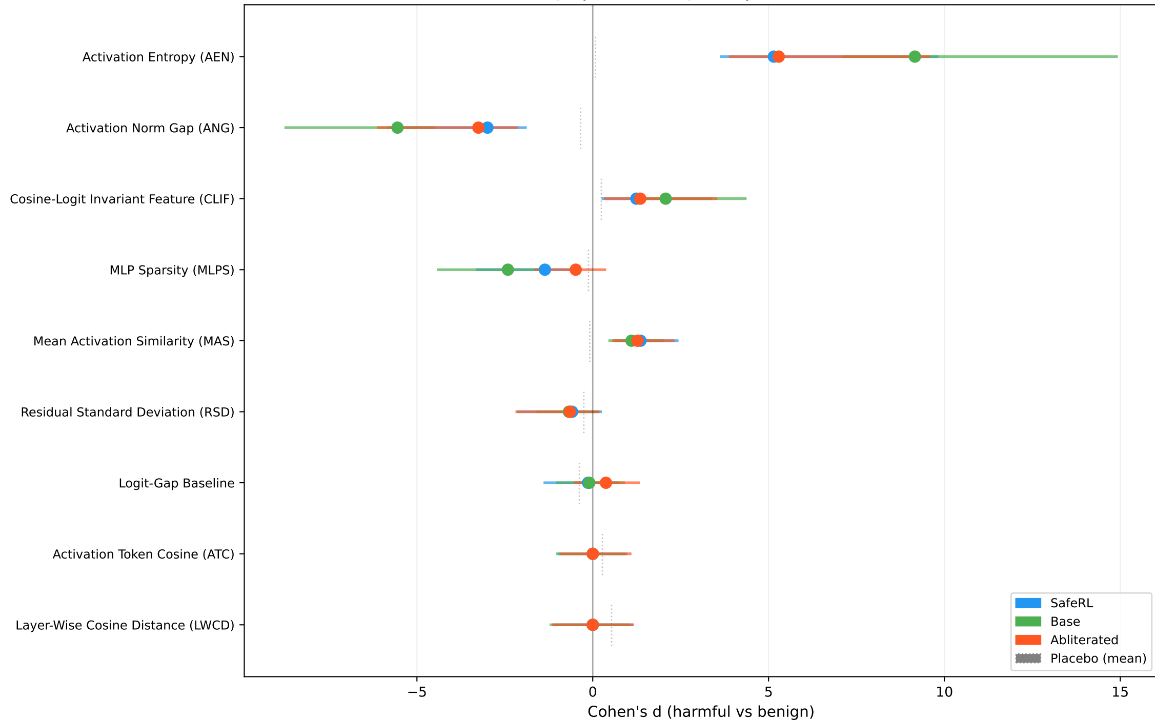
Forest Plot: Safety Metric Effect Sizes with 95% Bootstrap CI Qwen3-4B Lineage | n=10 per group | 1000 bootstrap resamples
