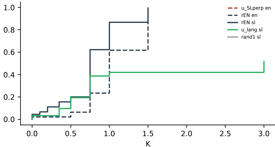
Gemma-3-12B-IT: per-prompt switch points (ECDF)
