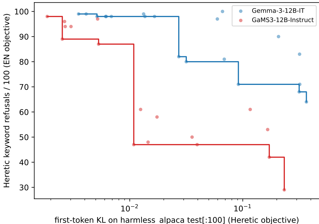
Heretic trials and Pareto fronts (NF4, reduced-trial)
