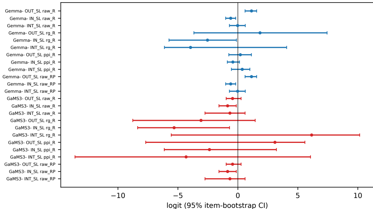
Output- vs input-side share of the edit-induced Slovene lag
