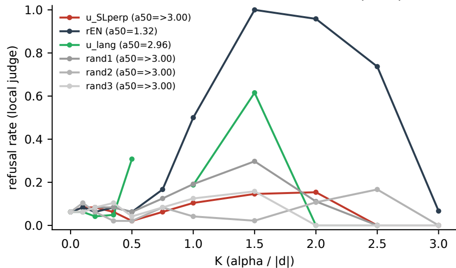
GaMS3-12B-Instruct - harmless EN-BT prompts
