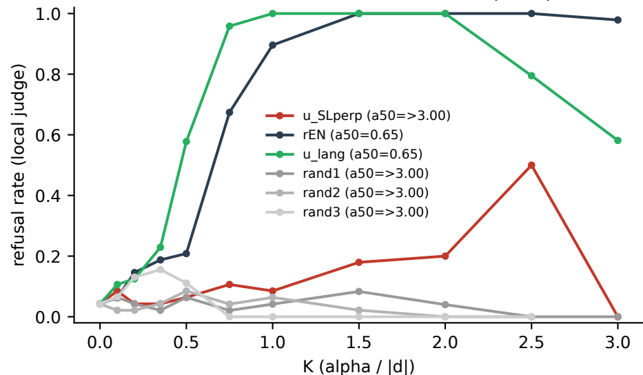
GaMS3-12B-Instruct - harmless SL-MT prompts
