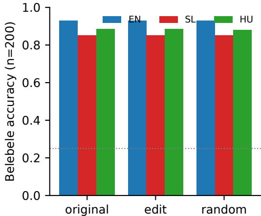
GaMS3-12B-Instruct
