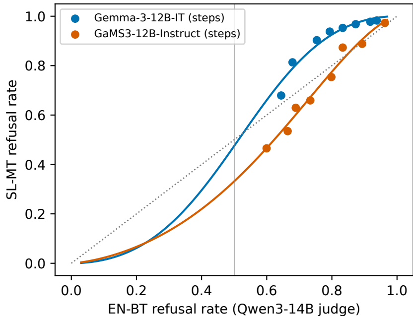
FINAL lambda curve; G3 = -0.60 [-1.31, 0.40]
