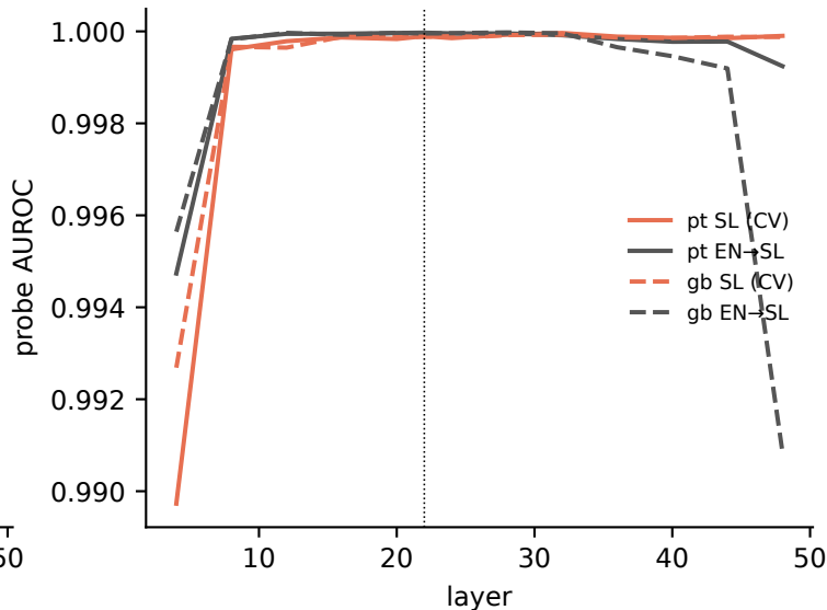
Probe AUROC (ceiling &gt;0.99 uninformative)
