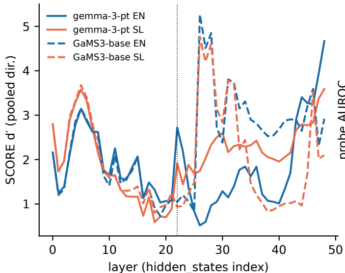
Base-model harm separability
