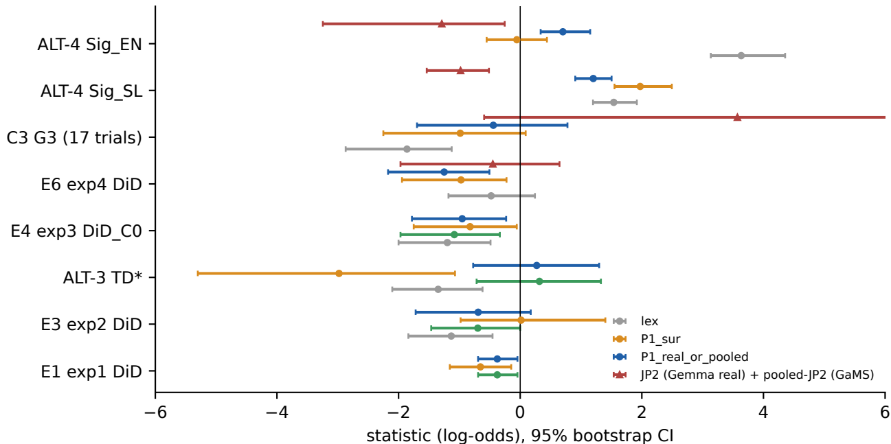
Readout sensitivity: the same saved responses, different refusal readouts
