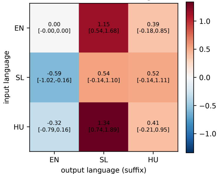
Gemma-3-12B-IT: L* (logit)
