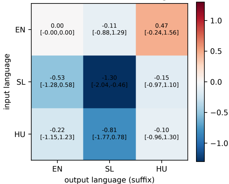
GaMS3-12B-Instruct: L* (logit)
