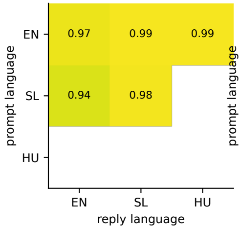
Gemma-3-12B-IT @ dose* (lo)
