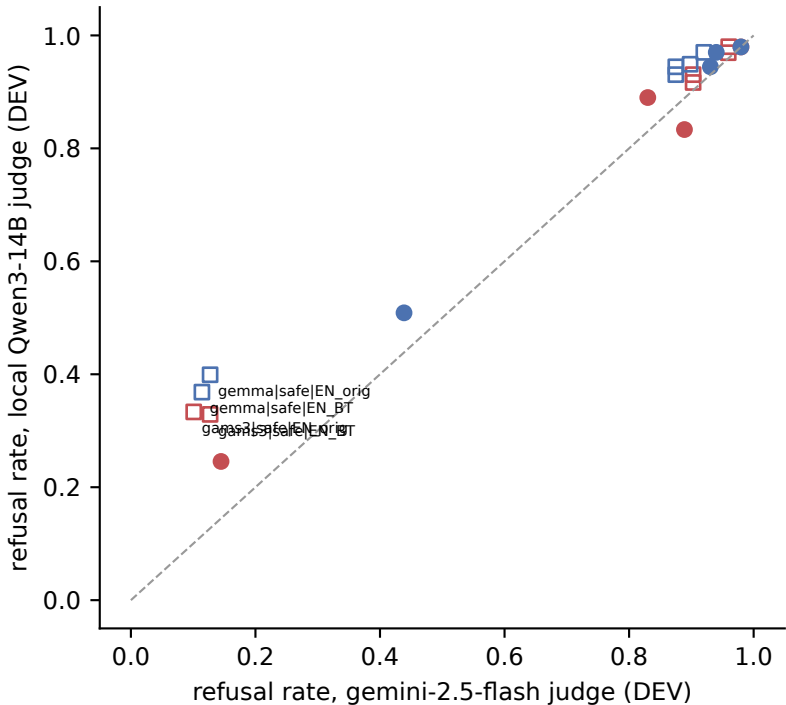
Judge calibration on DEV cells (filled = SL arm, open = EN arm; blue = Gemma, red = GaMS)
