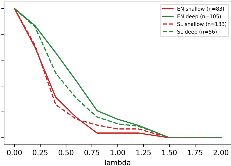
GaMS3-12B-Instruct
